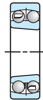
TAPERED BORE 1:12
