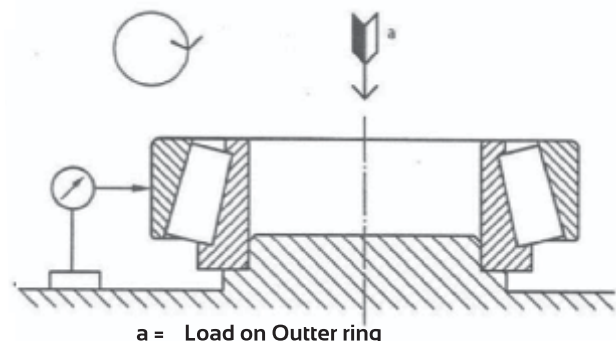
K_{ea} MEASUREMENT OF TAPER ROLLER BEARING
