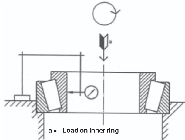
K_{ia} MEASUREMENT OF TAPER ROLLER BEARING
