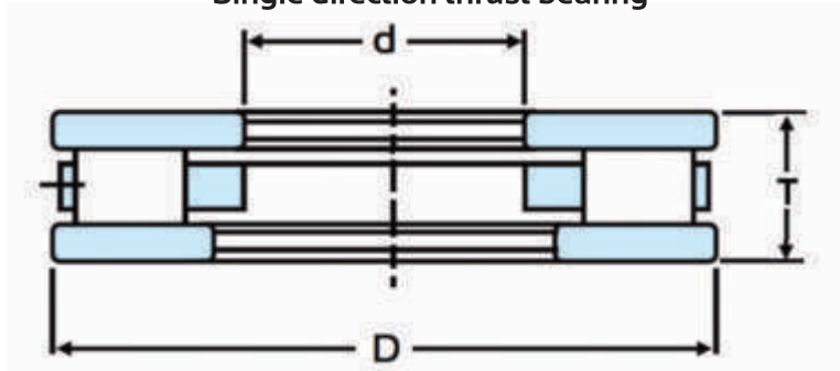
Single direction thrust bearing
