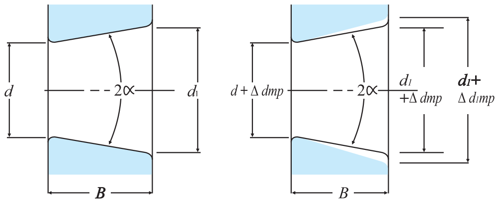
Tapered hole having dimensional difference of the average bore diameter within the flat surface
