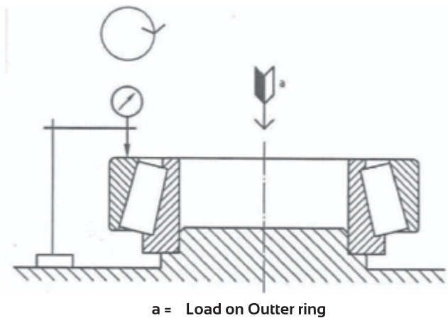
S_{ea} MEASUREMENT OF TAPER ROLLER BEARING
