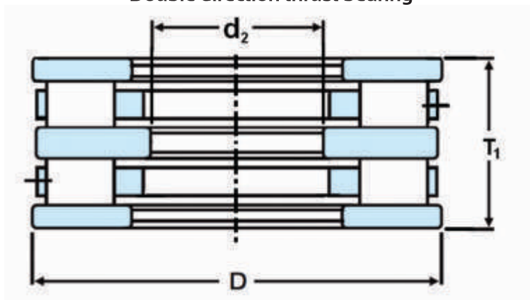
Double direction thrust bearing
