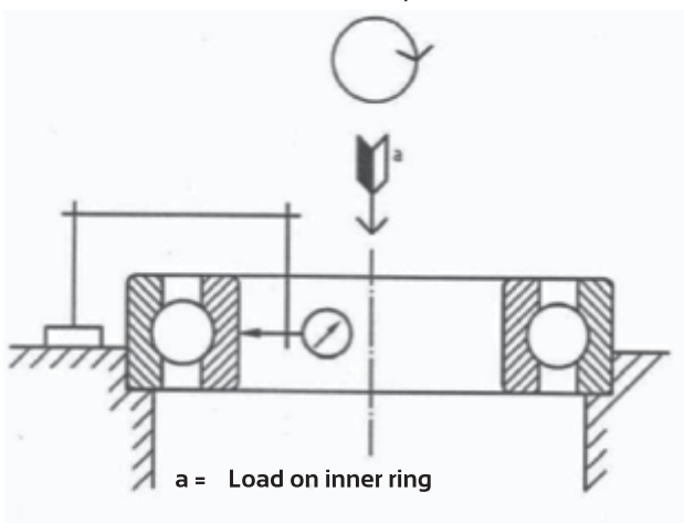
K_{ia} MEASUREMENT OF BALL BEARING
